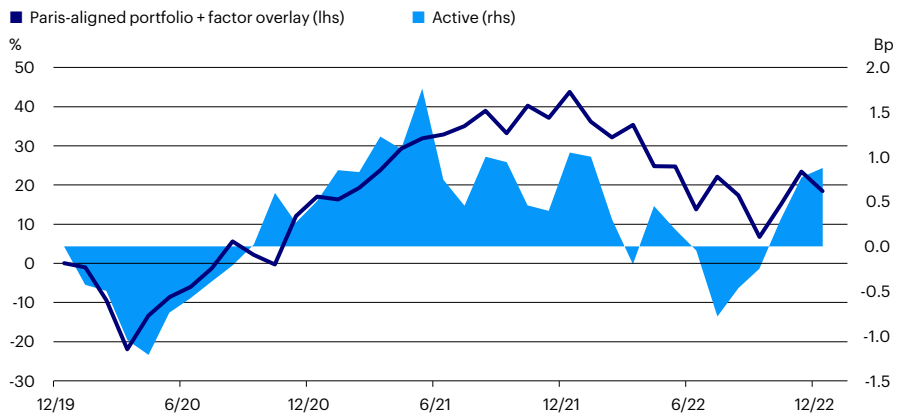
Figure 6 Cumulated portfolio performance and active return
