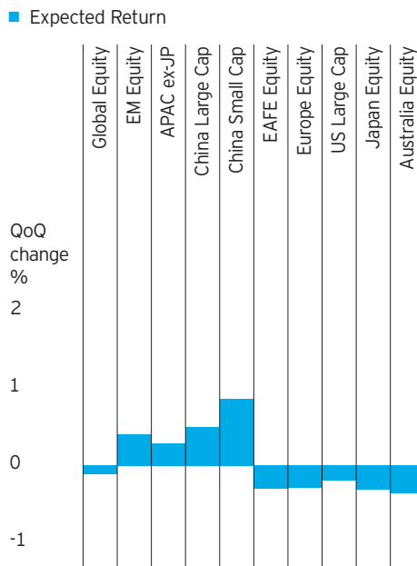
Figure 9: Equity year-over-year change (CNY)
