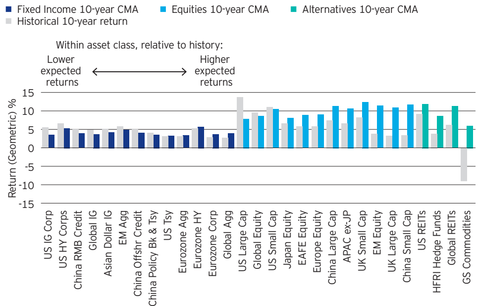
Figure 1: Expectations relative to historical average (CNY)
