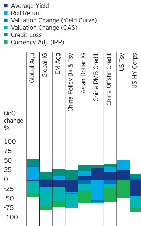
Figure 12: Fixed income year-over-year change attribution (CNY)
