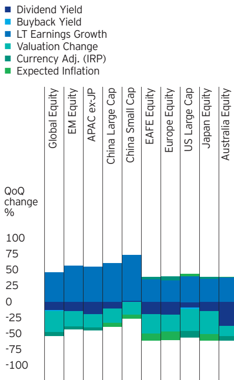
Figure 11: Equity year-over-year change attribution (CNY)
