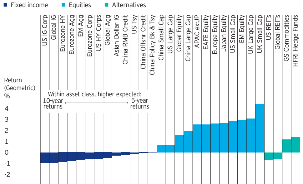
Figure 8: CMA difference: 5-year minus 10-year assumptions (CNY)
