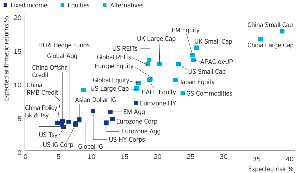
Figure 7: 10-year asset class expectations (CNY)
