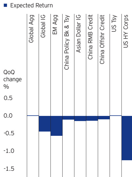
Figure 10: Fixed income year-over-year change (CNY)
