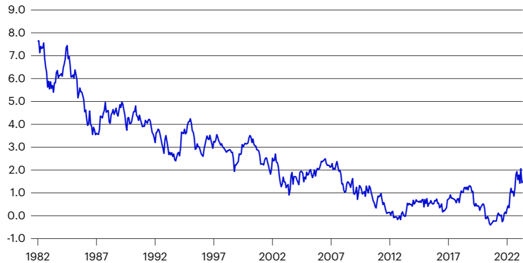
Figure 1.3 US 10-year real interest rate (%)
